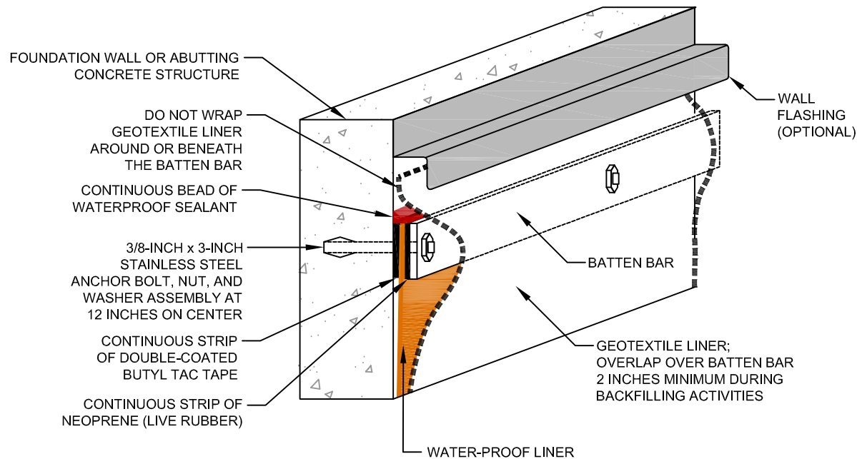
BATTEN BAR DETAIL (NOT TO SCALE)
