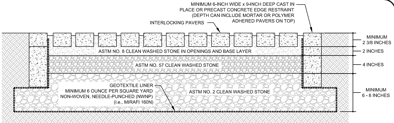
PERMEABLE PAVER DRIVEWAY - CROSS SECTION VIEW (NOT TO SCALE)
